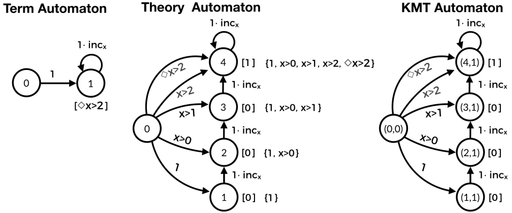
Fig. 17. Automata construction for \text{inc}_x^* \cdot \Diamond x > 2 in the theory of \text{LTL}_f(\text{IncNat}) .
